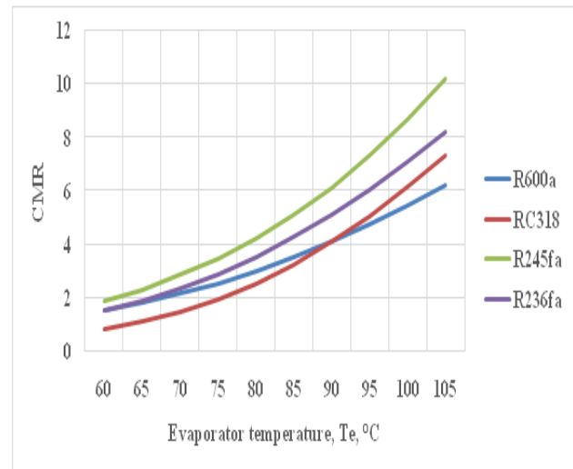
Figure 13: The effect of evaporator temperature on the CMR for various candidates in the basic ORC-VCR system.
