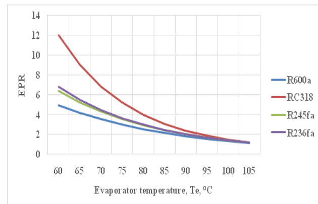
Figure 14: The effect of evaporator temperature on the EPR for various candidates in the basic ORC-VCR system.
