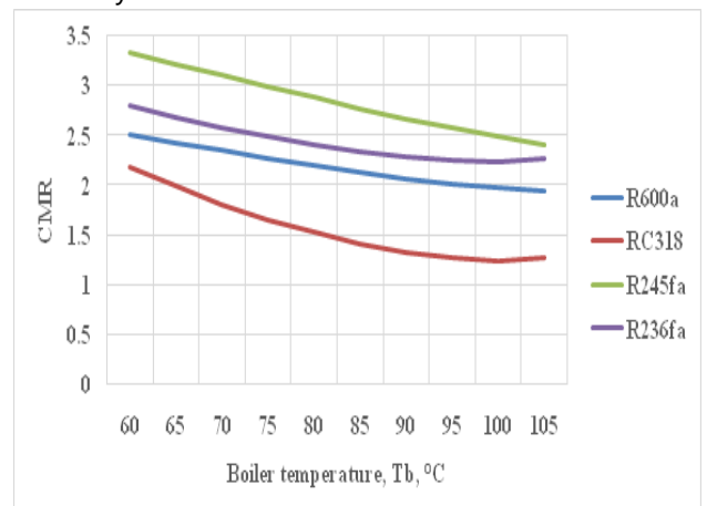
Figure 4: The effect of boiler temperature on the CMR for various candidates in the basic ORC-VCR system.
