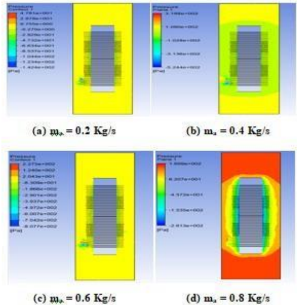
Fig 7. Pressure contour plot for different flow rates and with trapezoidal fin.
