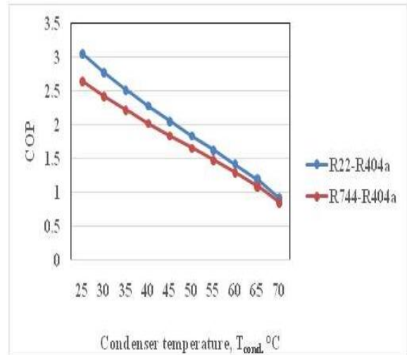
Fig. 6: Effect of condenser temperature on COP.
