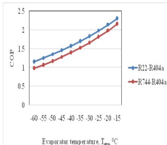
Fig. 2: Effect of evaporator temperature on COP.
