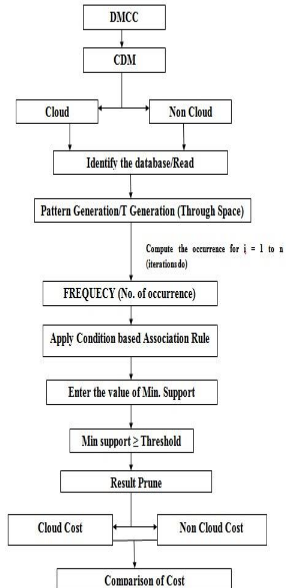
Figure 3 Flowchart of CDM
