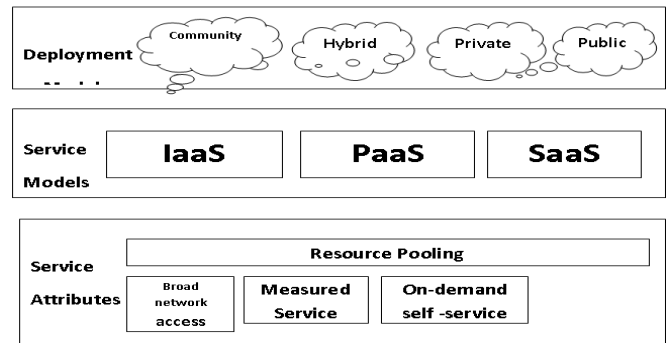
Figure 1 Cloud Computing
