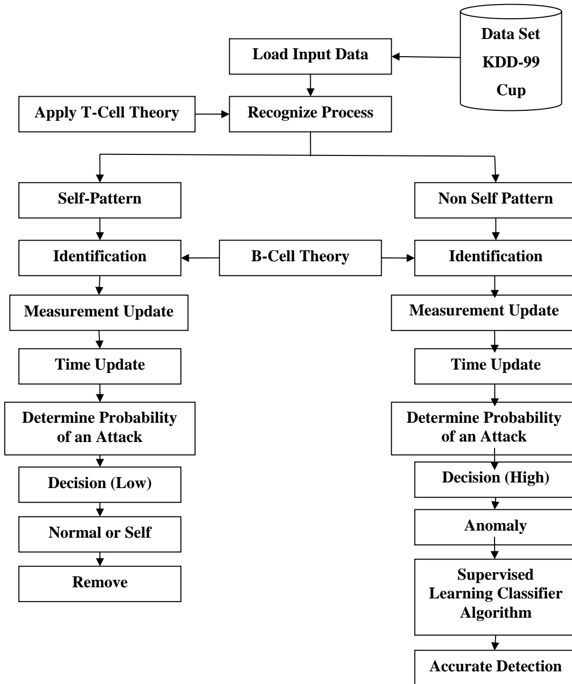
Figure 1 Model Flow Design Chart of proposed Methodology
