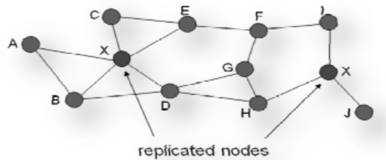
Figure1. Replication Attack
