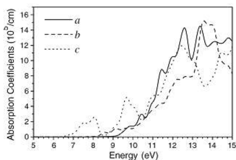
Figure 3. Linear absorption coefficients of PVDF.
